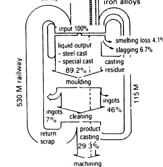
⑦ Materials flow - quantitative
